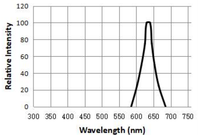
Spectrum Distribution (Ta=25°C)
