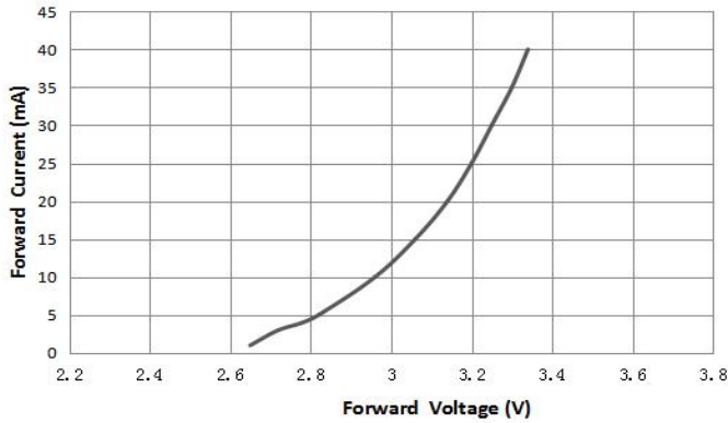
Forward Current VS. Forward Volutag (Ta=25°C)
