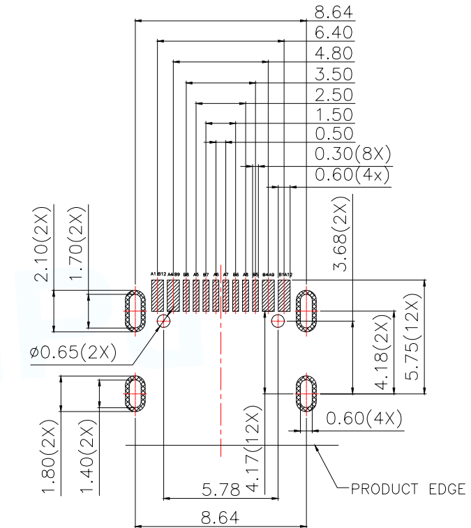
RECOMMENDED PCB LAYOUT(TOP VIEW) THICKNESS 1.00MM;DEFAULT TOLERANCE:±0.05
