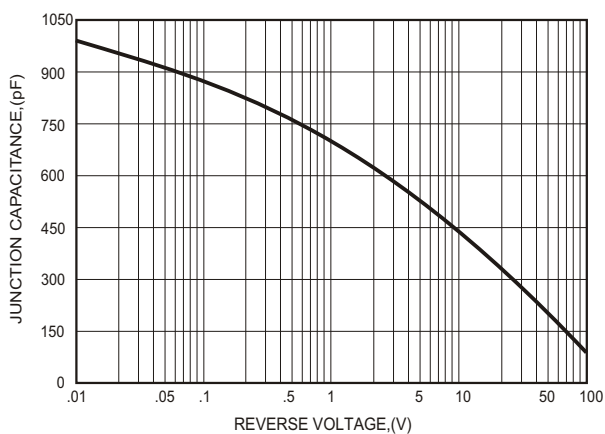
FIG.5-TYPICAL JUNCTION CAPACITANCE
