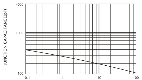
FIG.5-TYPICAL JUNCTION CAPACITANCE
