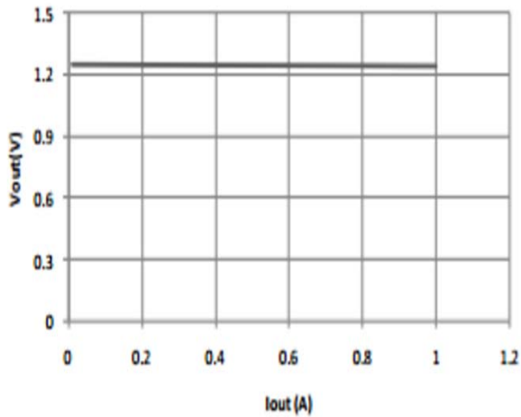
AMS1117-ADJ Vout Vs. Iout
