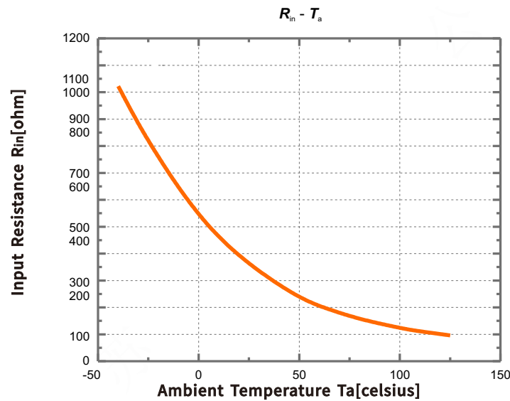
Figure 2. Input resistance R_{in} as a function of ambient temperature T_a .
