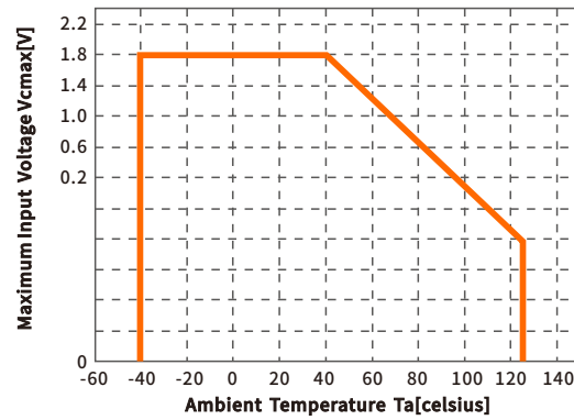
Figure 1.2 Maximum input Voltage V_{cmax}
