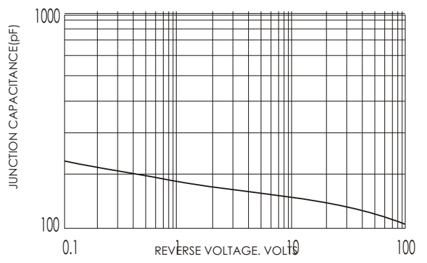
FIG.5-TYPICAL JUNCTION CAPACITANCE
