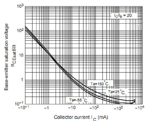
Figure 6. Equivalent on-resistance
