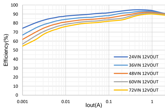
Efficiency, Vout=12V
