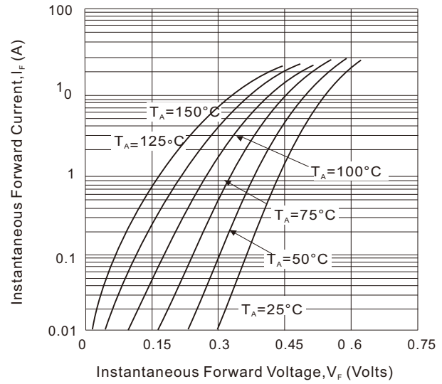
FIG.2-TYPICAL FORWARD CHARACTERISTICS
