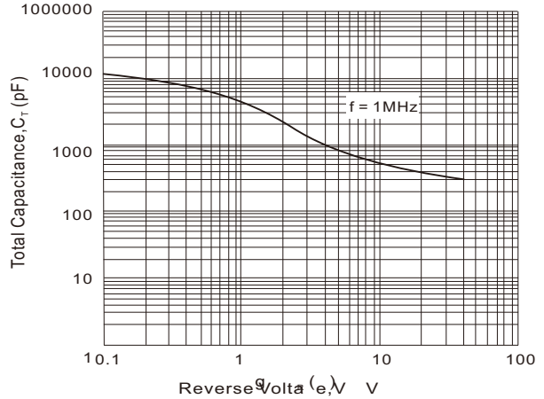
FIG.5-TYPICAL JUNCTION CAPACITANCE
