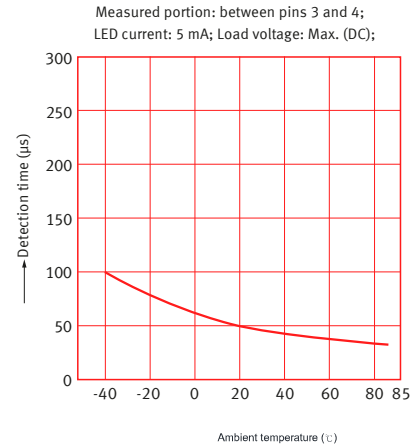
Detection time vs. ambient temperature characteristics
