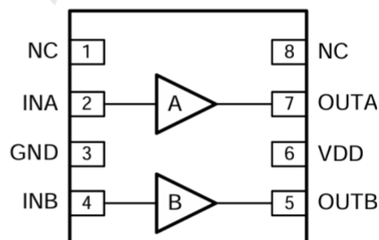
DUAL NONINVERTING
