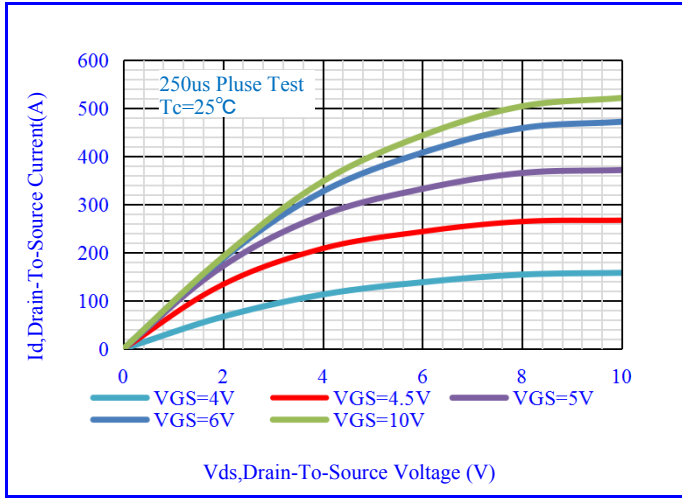
Fig.1-Output Characteristics
