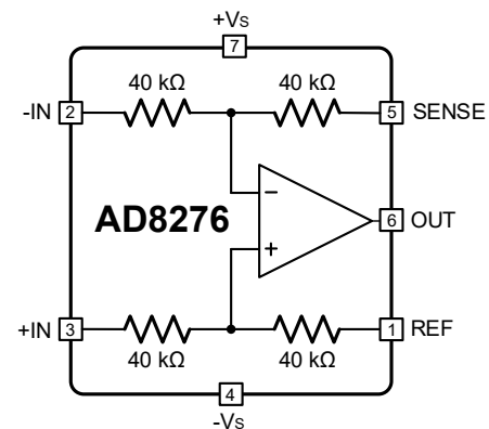
Figure 2. AD8276
