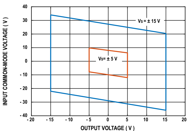
Figure 16. Input Common-Mode Voltage vs. Output Voltage ( \pm 15 V and \pm 5 V Supplies)
