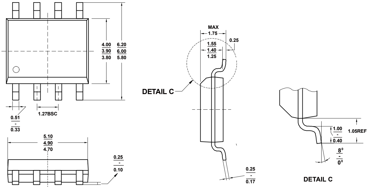
Figure 54. 8-Lead SOIC Package Dimensions shown in millimeters
