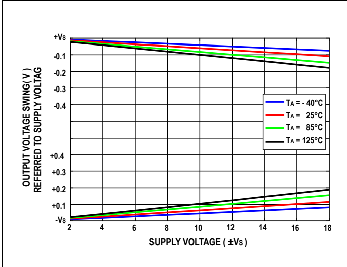
Figure 20. Output Voltage Swing vs. Supply Voltage and Temperature ( R_L = 10 k \Omega )
