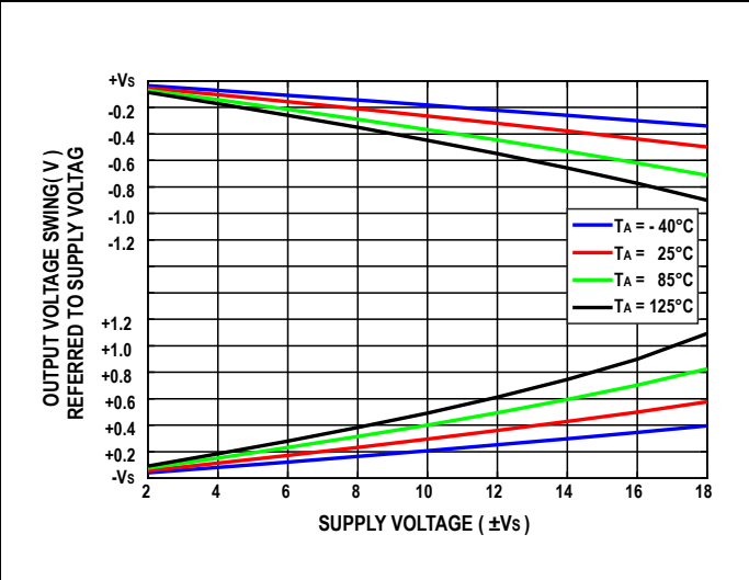
Figure 19. Output Voltage Swing vs. Supply Voltage and Temperature ( R_L = 2 k \Omega )
