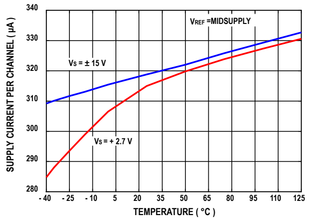
Figure 27. Supply Current per Channel vs. Temperature
