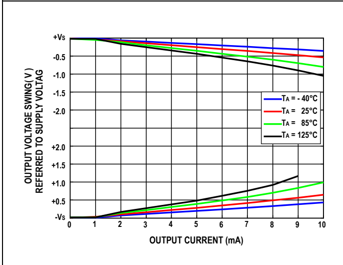
Figure 22. Output Voltage Swing vs. Output Current and Temperature ( V_S = \pm 15 V)
