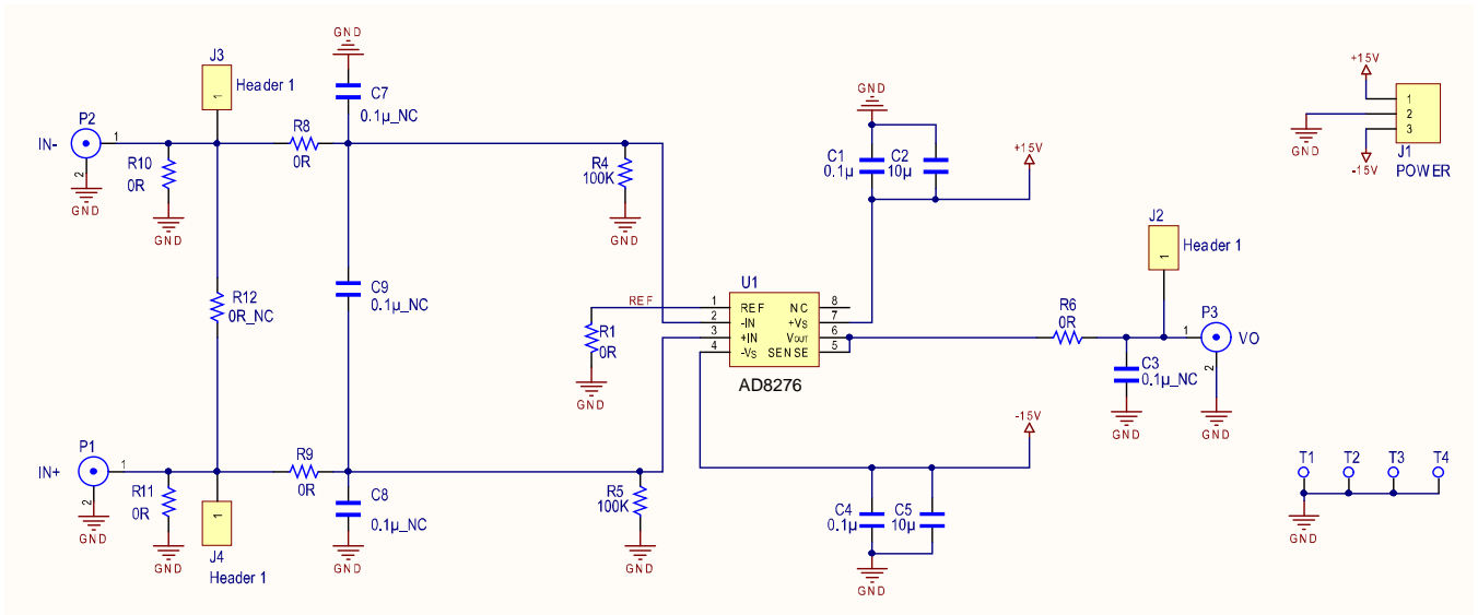
Figure 51. AD8276 Evaluation Board Schematic
