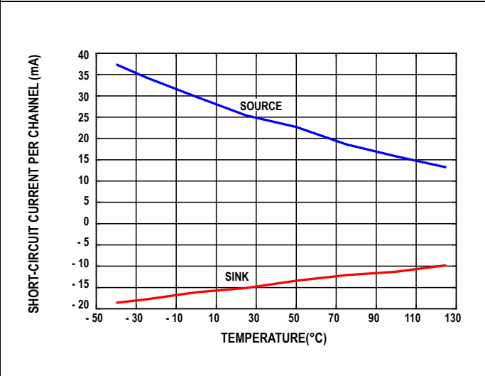
Figure 23. Short-Circuit Current per Channel vs. Temperature
