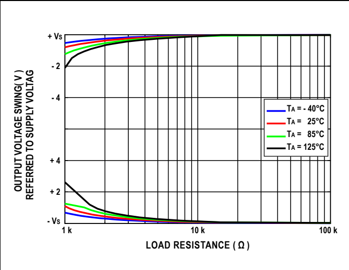
Figure 21. Output Voltage Swing vs. Load Resistance and Temperature ( V_S = \pm 15 V)
