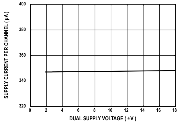
Figure 25. Supply Current per Channel vs. Dual Supply Voltage ( V_{IN} = 0 V )
