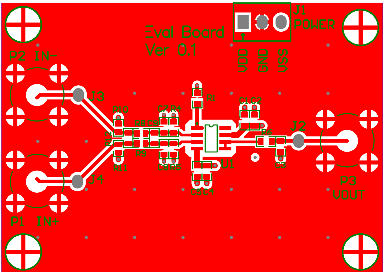
Figure 52. Layout of AD8276 Evaluation Board (Top Layer)
