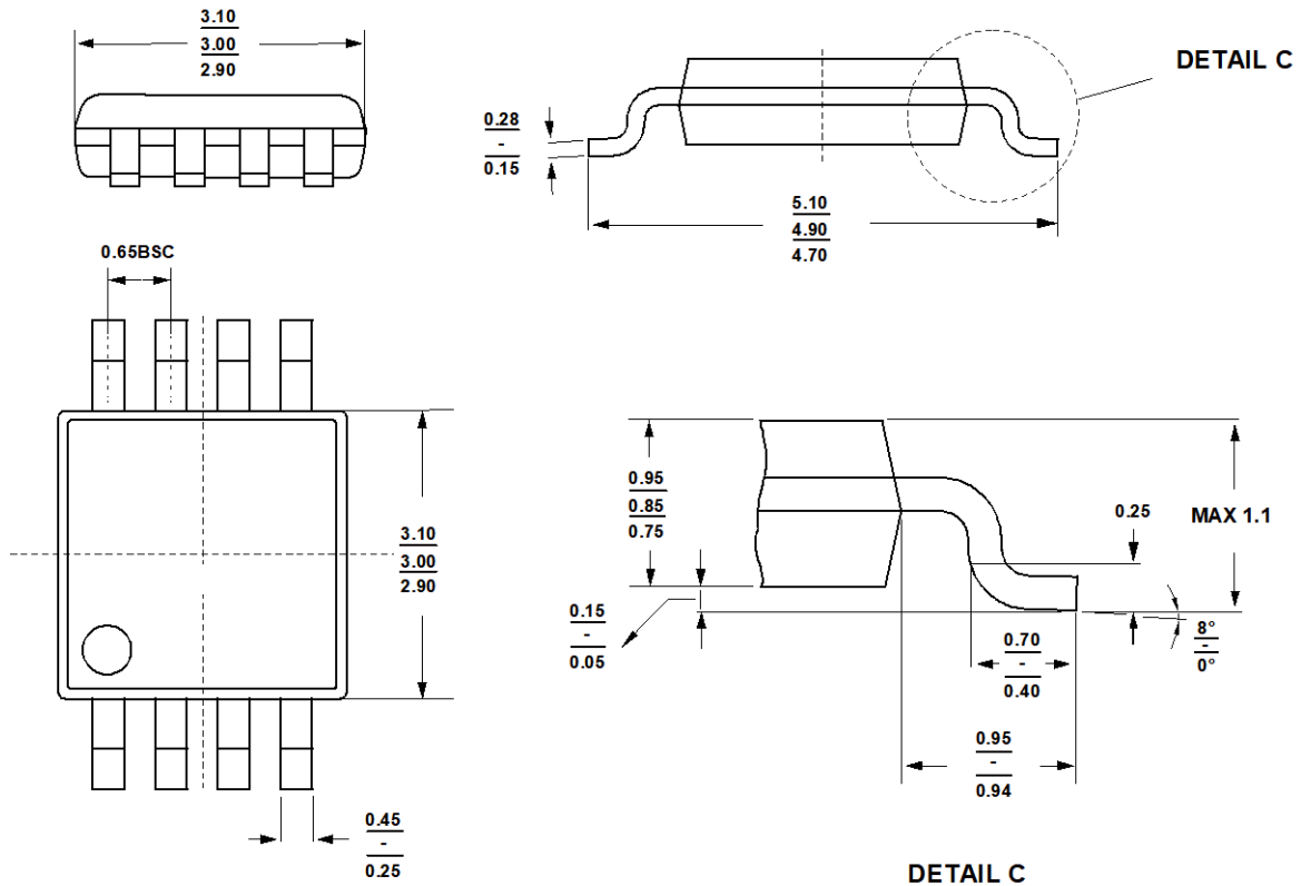
Figure 55. 8-Lead MSOP Package Dimensions shown in millimeters
