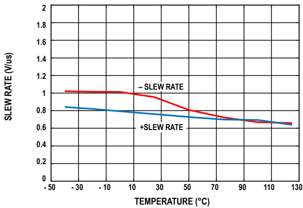
Figure 24. Slew Rate vs. Temperature ( V_{IN} = 20 V_{P-P} , 1 kHz)
