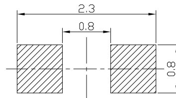
推荐焊盘尺寸 Recommended Soldering Pad
