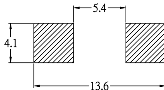
Recommend Land Pattern Dimensions
