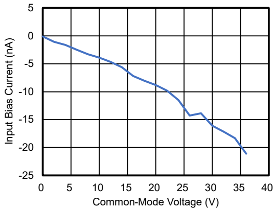
Figure 3. Input Bias Current vs. Common-Mode Voltage (Enabled)
