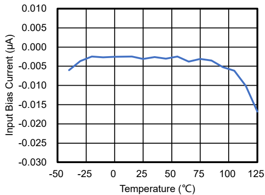
Figure 5. Input Bias Current vs. Temperature (Enabled)
