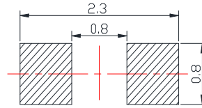
推荐焊盘尺寸 Recommended Soldering Pad
