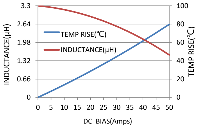
MAWH-1770-3R3-M-5A
