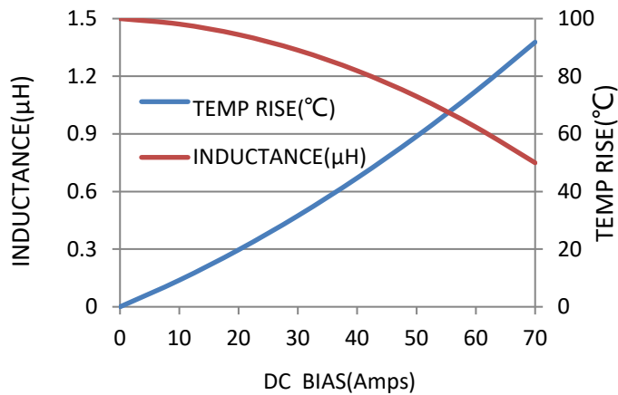
MAWH-1770-1R5-M-5A
