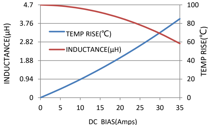
MAWH-1770-4R7-M-5A
