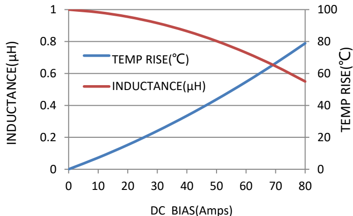
MAWH-1770-1R0-M-5A
