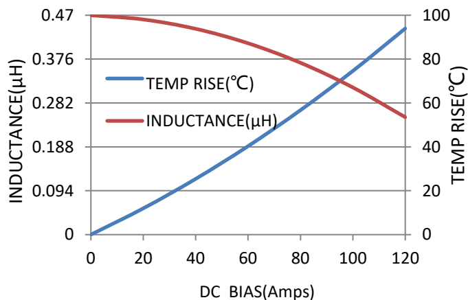
MAWH-1770-R47-M-5A
