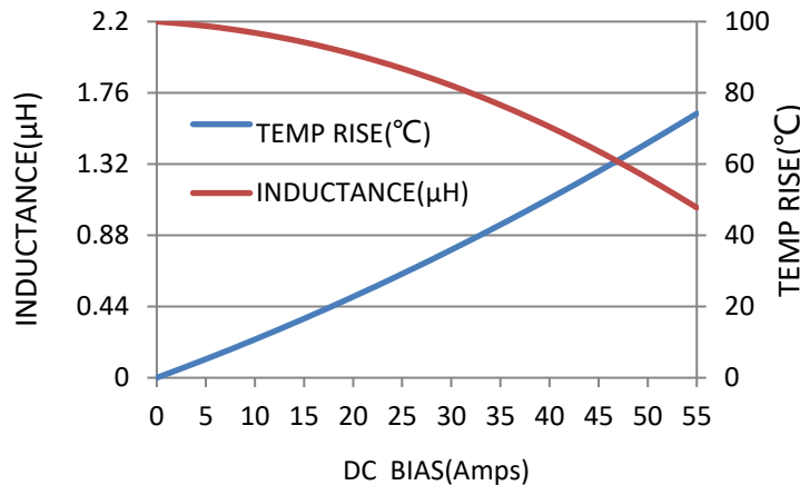
MAWH-1770-2R2-M-5A
