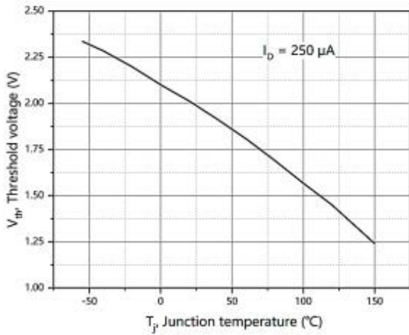
Figure 7. Threshold voltage
