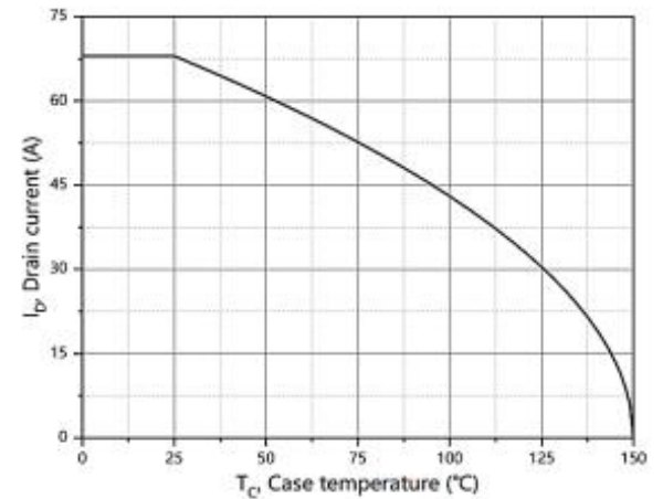
Figure 10. Drain current
