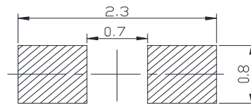
推荐焊盘尺寸 Recommended Soldering Pad
