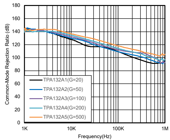
Figure 7. Common-Mode Rejection Ratio vs. Frequency
