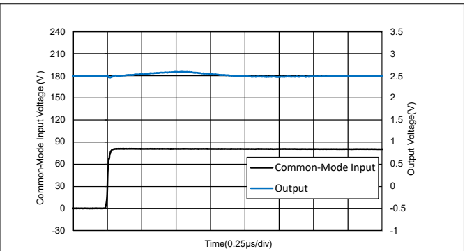
Figure 15. Common-Mode Voltage Transient Response
