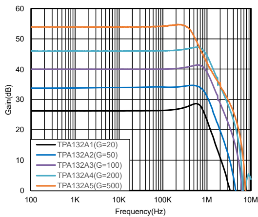
Figure 6. Gain vs. Frequency
