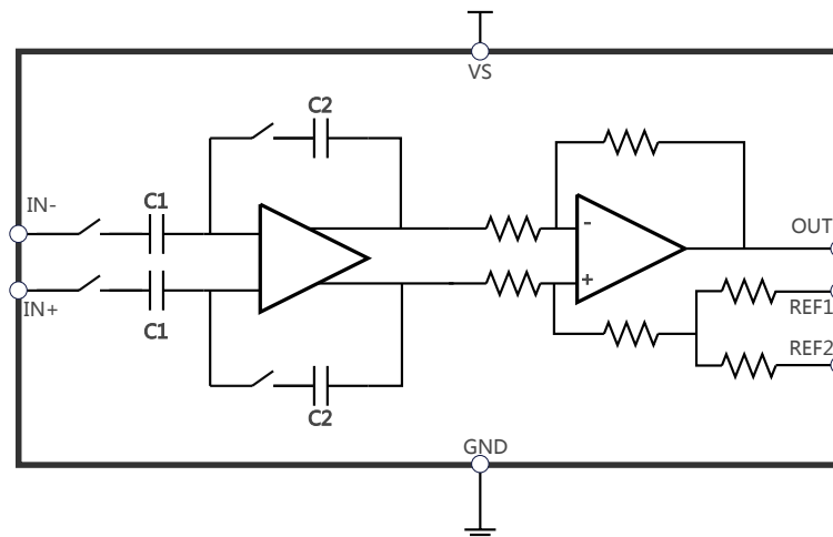
Figure 22. Brief Circuit Diagram of TPA132
