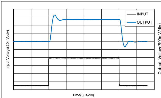
Figure 14. Step Response
