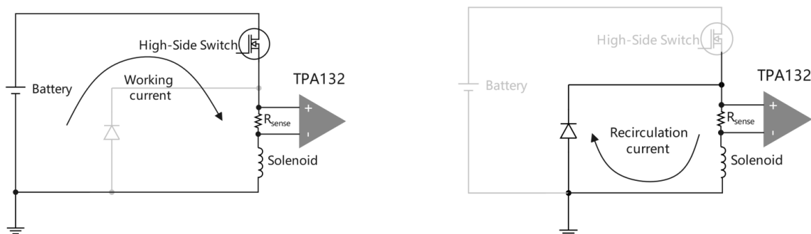
Figure 19. Solenoid Application Circuits
