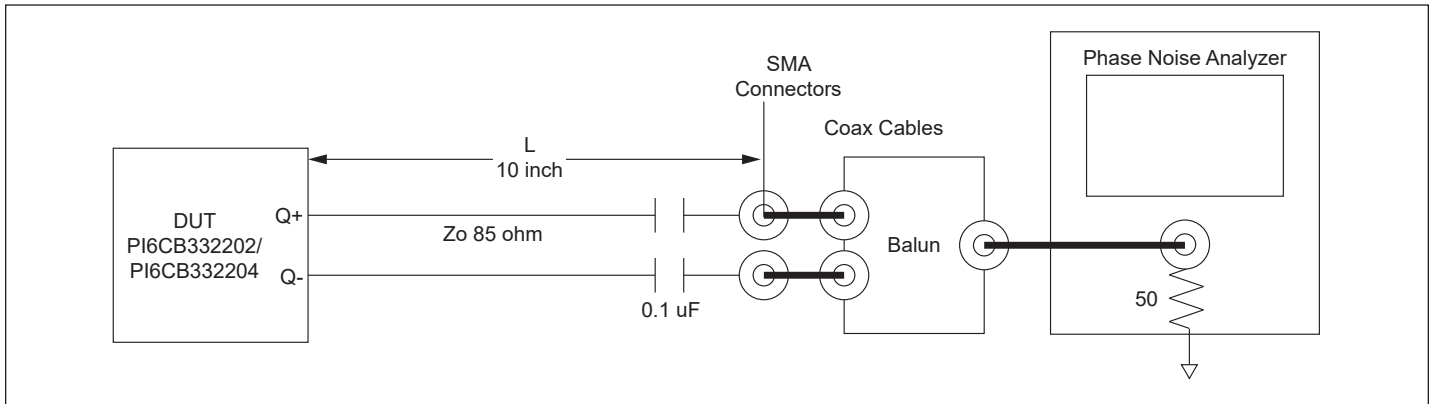
Figure 5. Test Set Up for Phase Jitter Measurement
