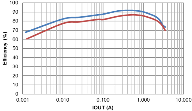
Figure 4. Efficiency vs. Output Current, V_{IN} = 12\text{V}
