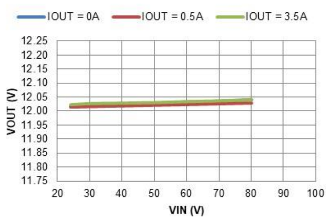
Figure 7. Line Regulation
