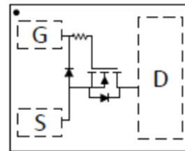
Top View Equivalent Circuit
