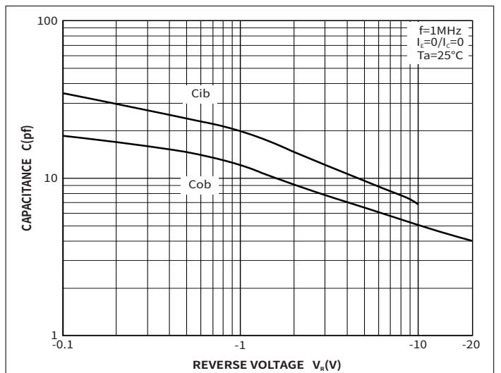
Fig.6 C_{ob}/C_{ib}-V_{CB} V_{EB}
