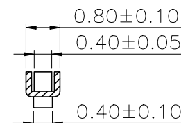
SEC: C-C
