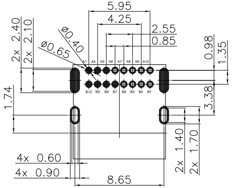
RECOMMENDED PCB LAYOUT(TOP) TOLERANCES: ±0.05MM
