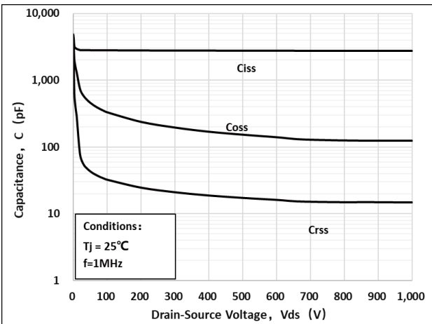
Fig 15: Capacitance Characteristics
