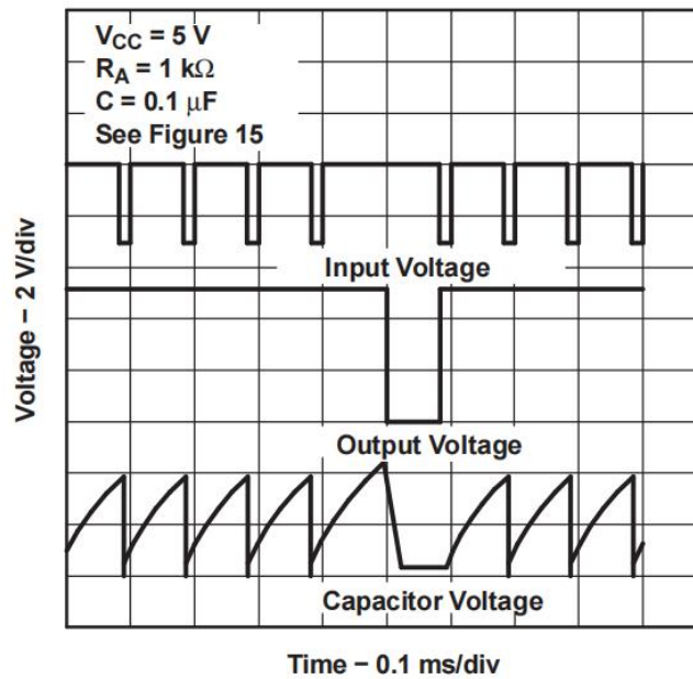
Figure 9. Completed Timing Waveforms for Missing-Pulse Detector
