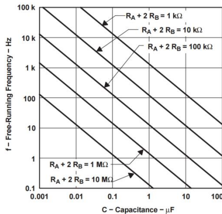
Figure 6. Free-Running Frequency
