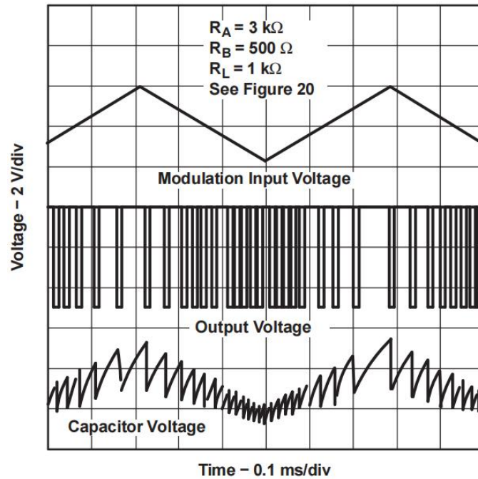
Figure 13. Pulse-Position-Modulation Waveforms
