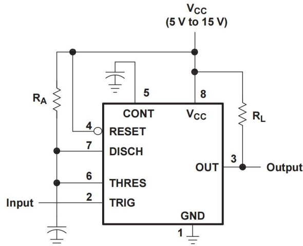
Figure 1. Circuit for Monostable Operation
