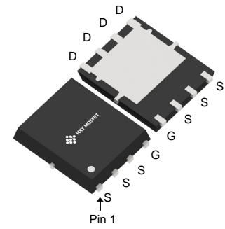
DFN5X6-8L
