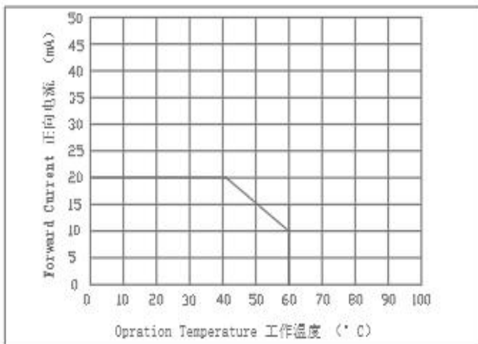
Max. Permissible Forward Current I_F = f(T)
