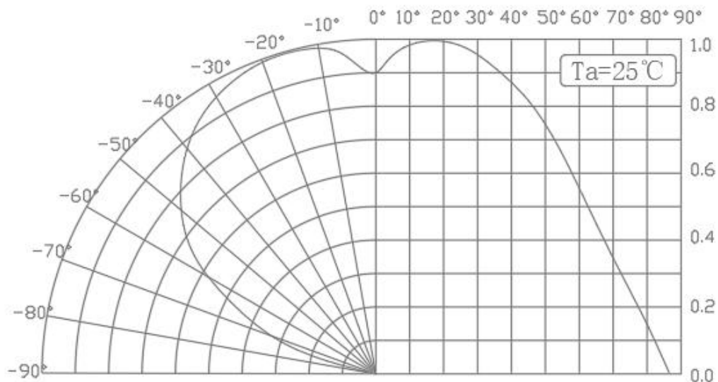
View angle VS. Radiation 半功率角VS. 发光强度曲线
