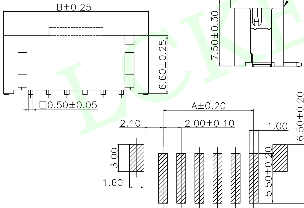
PCB LAYOUT
