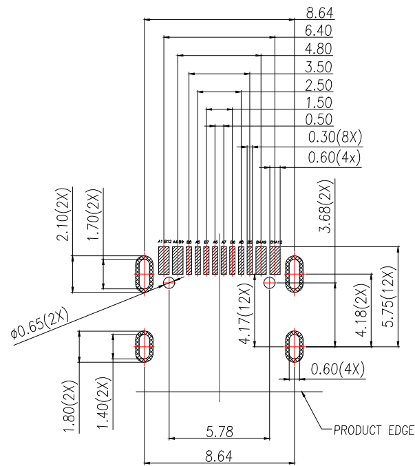
RECOMMENDED PCB LAYOUT(TOP VIEW) THICKNESS 1.00MM;DEFAULT TOLERANCE:±0.05
