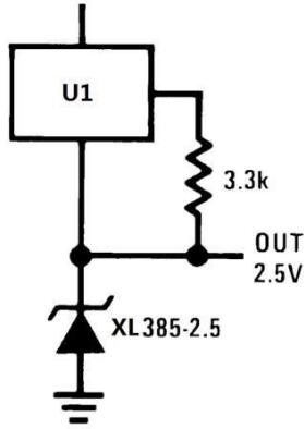
Figure 13. Wide Input Range Reference
