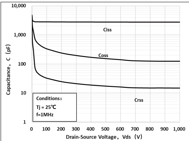
Fig 15: Capacitance Characteristic
