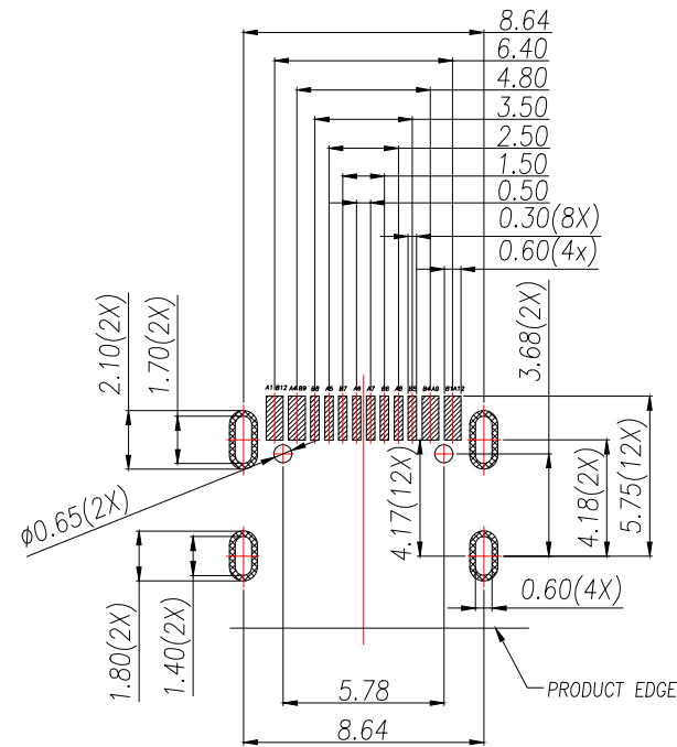
RECOMMENDED PCB LAYOUT(TOP VIEW) THICKNESS 1.00MM;DEFAULT TOLERANCE:±0.05
