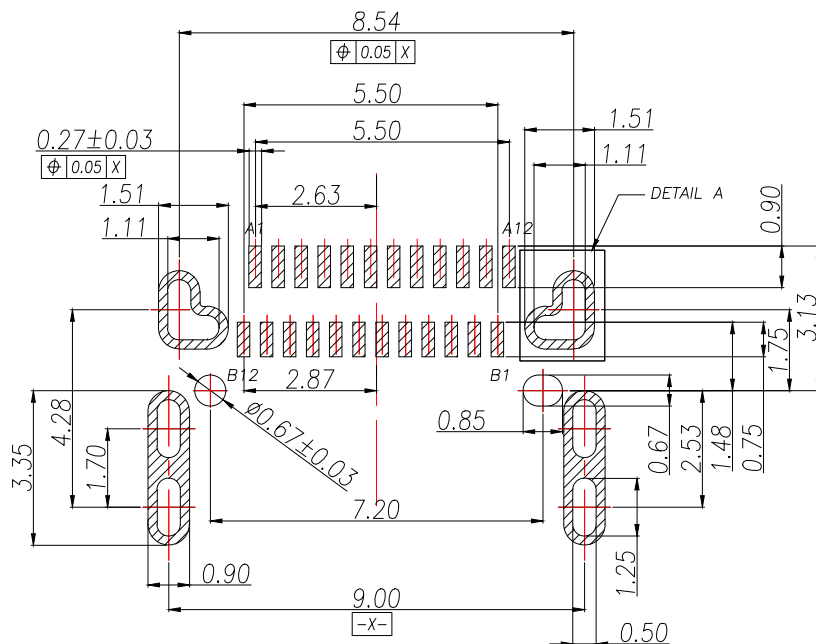
SCALE 2:1 RECOMMENDED PCB LAYOUT(TOP VIEW) Thickness 1.0mm (TOLERANCE=±0.05mm)
