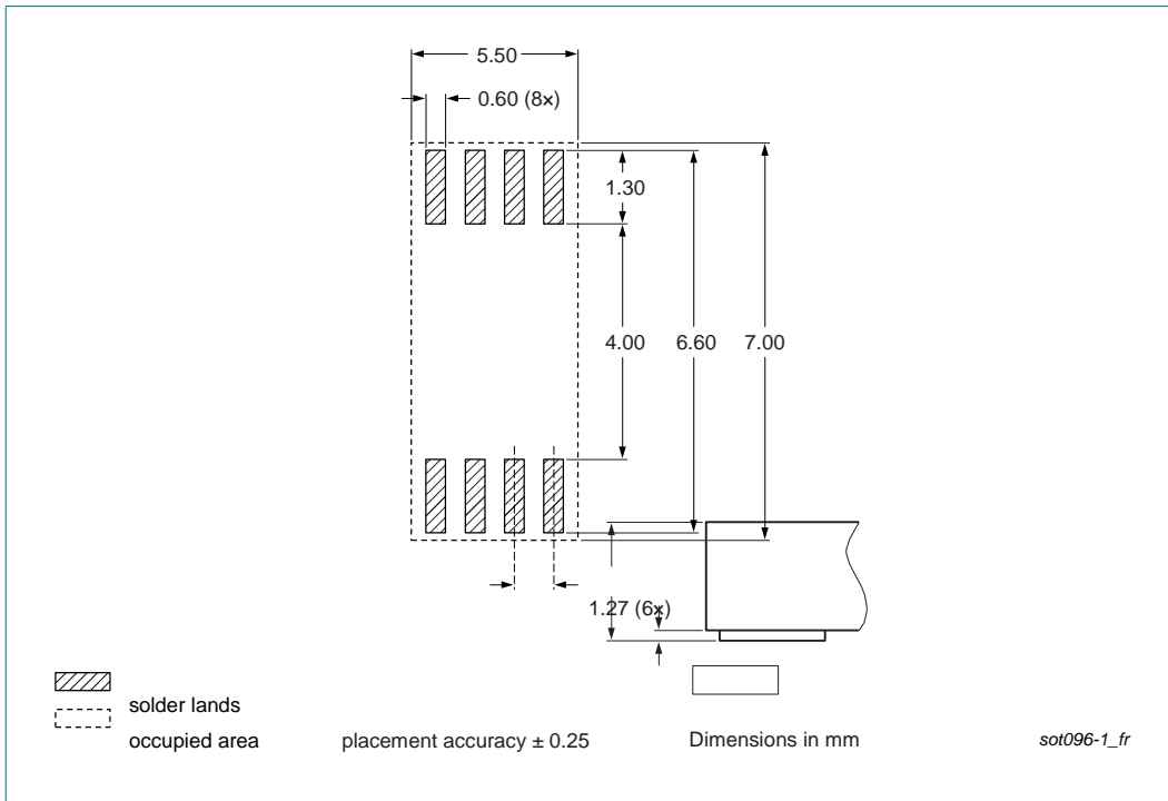
Fig 22. PCB footprint for SOP8
