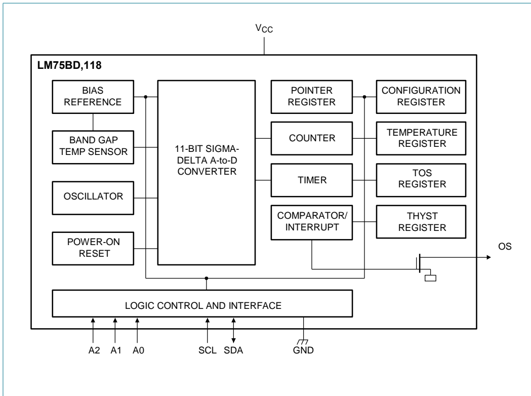
Fig 1. Block diagram of LM75BD,118
