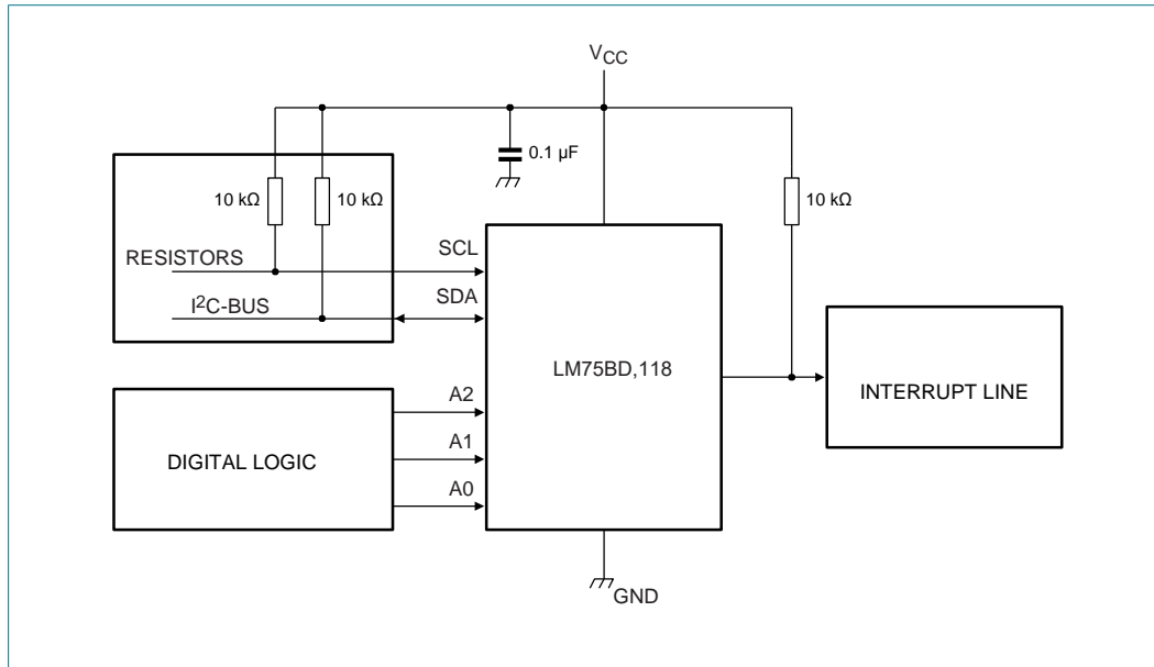
Fig 13. Typical application
