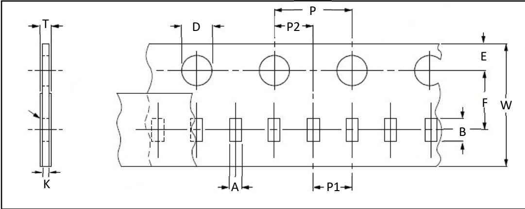
纸带结构 Structure of paper tape.
