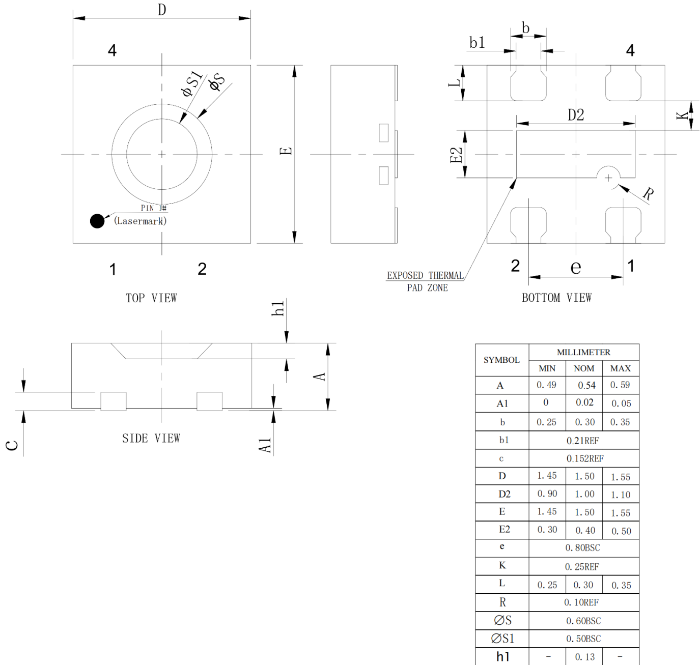
Figure 7 Dimensional drawing of SHT40-AD1F-R2 (in mm)
