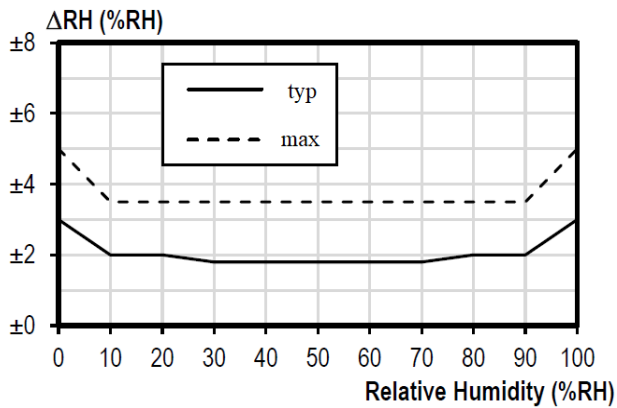
Figure 2 SHT40-AD1F-R2 RH accuracy @25°C
