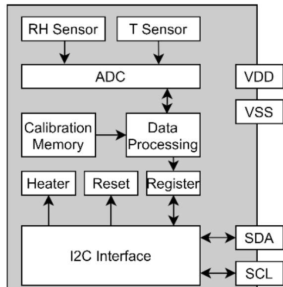
Functional Block Diagram of SHT40-AD1F-R2
