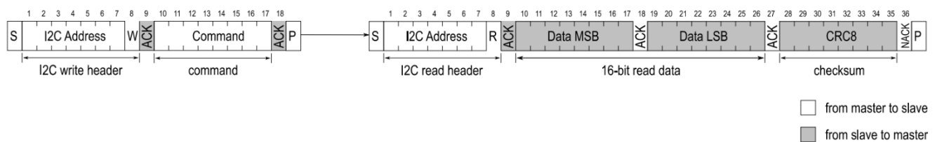
Figure 5 Typical I 2 C communication timing of SHT40-AD1F-R2
