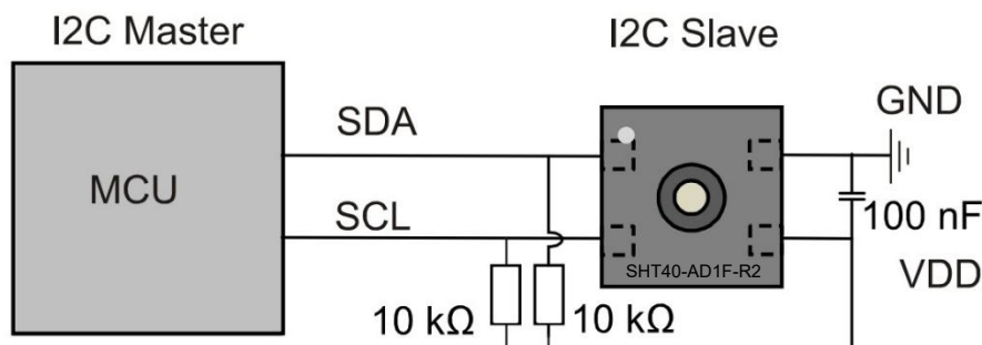
Figure 6 Typical application circuit reference diagram of SHT40-AD1F-R2
