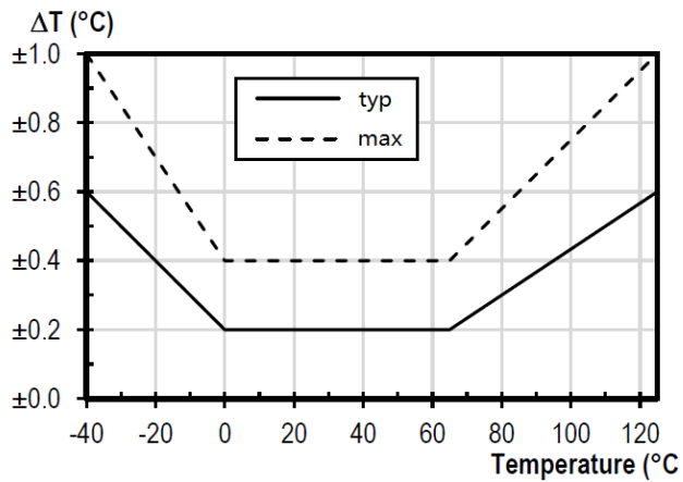
Figure 4 SHT40-AD1F-R2 temperature accuracy
