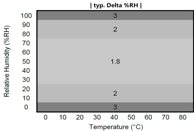
Figure 3 Typical RH accuracy tolerance over humidity and temperature for SHT40-AD1F-R2
