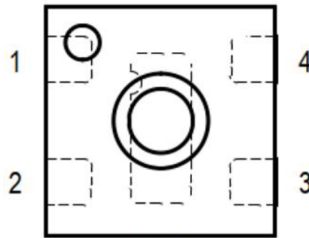
Figure 1 Top View of SHT40-AD1F-R2
