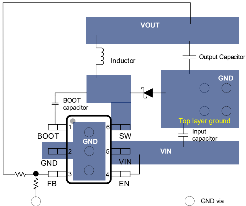
Figure 10. Layout Example
