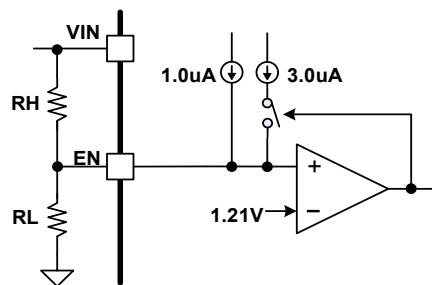
Figure 12. System UVLO by EN divider
