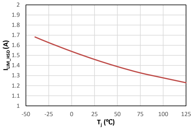
Figure 9. Switch Current Limit vs Junction Temperature
