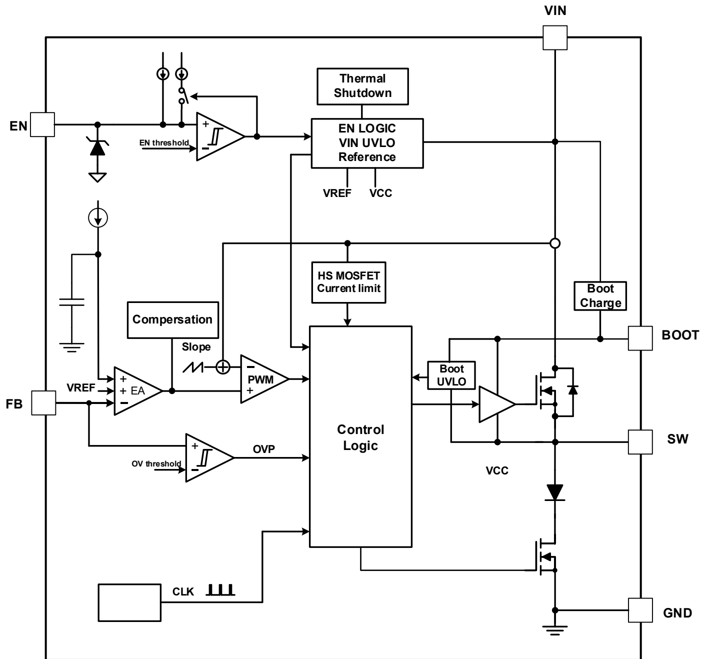
Figure 11. Block Diagram of LMR16006
