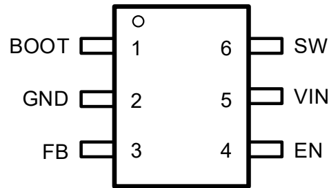
Top View: LMR16006XDDCR TSOT23-6L
