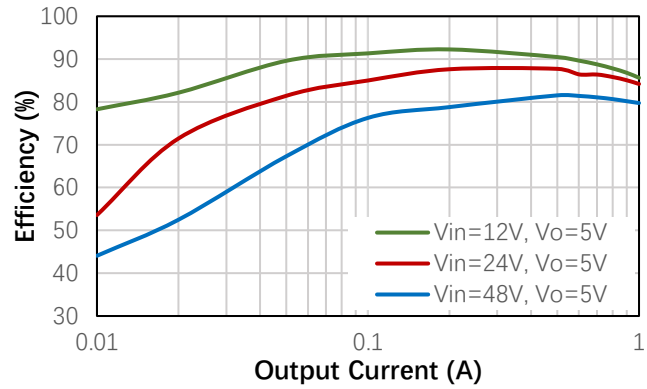
Figure 2. Power Efficiency
