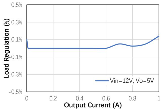
Figure 6. Load Regulation
