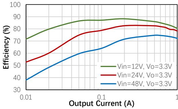
Figure 1. Power Efficiency
