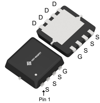
DFN3X3-8L DFN-8(3x3)
