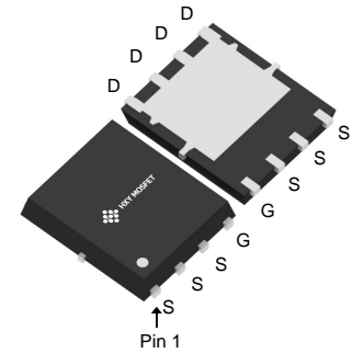
DFN5X6-8L (PQFN-8(5x6))
