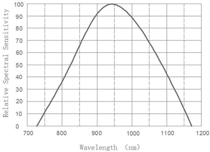
Spectral Sensitivity
