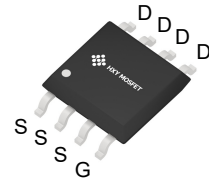
SOP-8 (SOIC-8)
