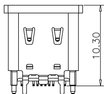
WITH PICK UP COVER SCALE 1:2
