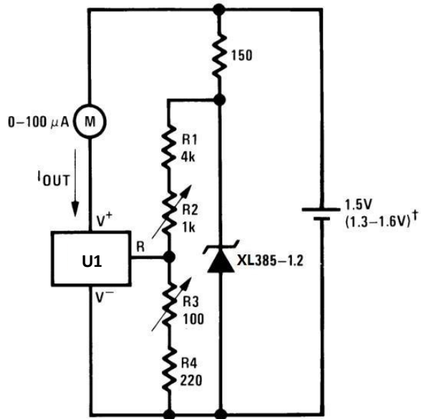
Figure 20. 20.0°C-100°C Thermometer
