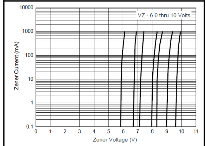
Figure 4: Typical Zener Breakdown Characteristics
