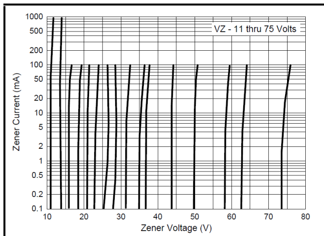
Figure 3: Typical Zener Breakdown Characteristics
